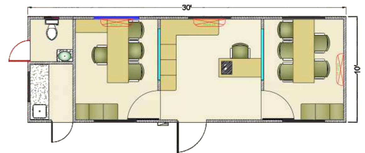
Sizes-30' x 10' 2 Executive Cabin & 1 Reception with WC & Pantry
