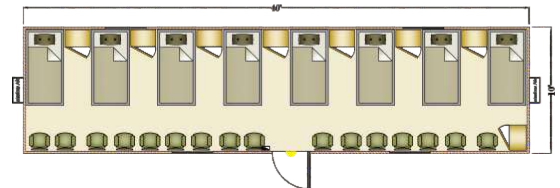
Sizes-40' x 10' 8 Person Accommodation with Locker
