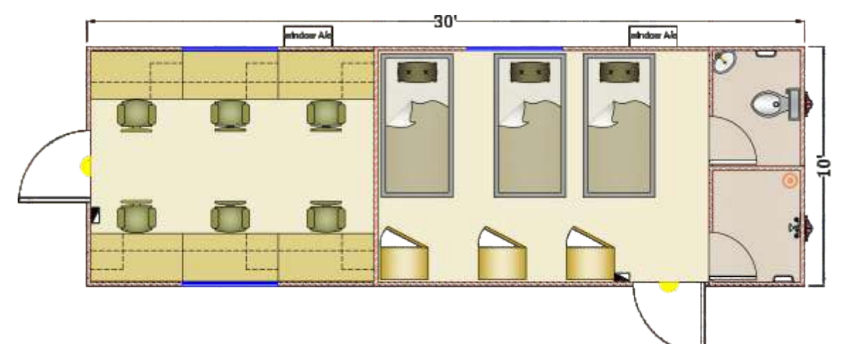
Sizes-30' x 10' 3 Person Accommodation with 6 Person Work Station WC + Washroom
