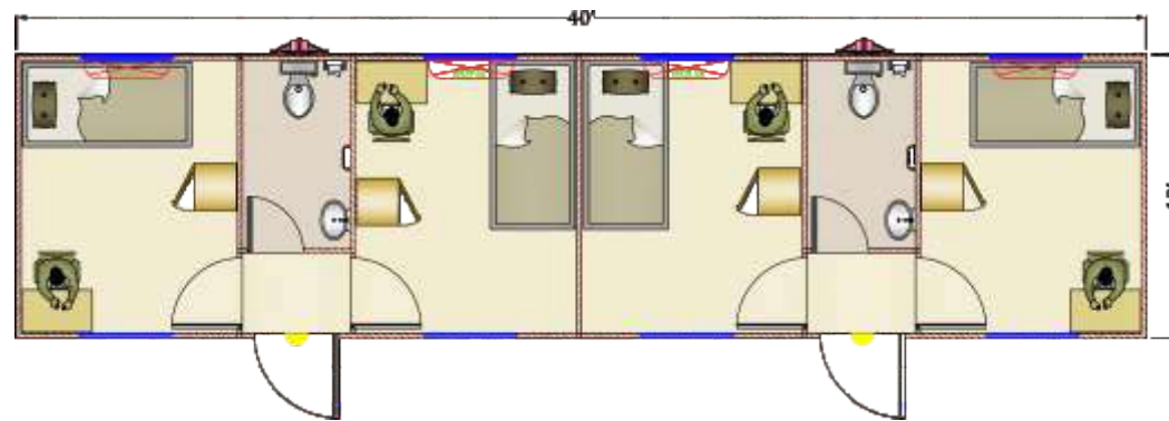
Sizes-40' x 10' 4 Person Accommodation with 2 WC + 2 Washroom
